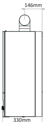
Figure 6 b (24 kW side)
