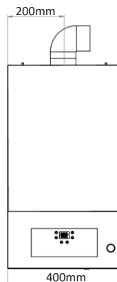
Figure 6 c (28-35 kW Front)
