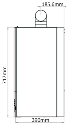
Figura 6 c (28-35 kW lateral)
