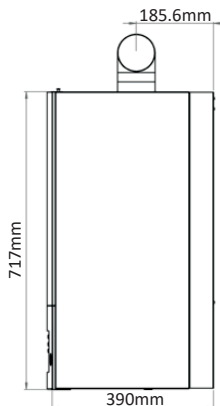
Figure 6 c (28-35 kW Side)
