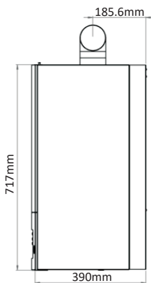
Figura 6 c (28-35 kW lateral)
